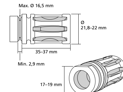
Required dimensions of NATO A1/A2 flash hiders for QM2.
